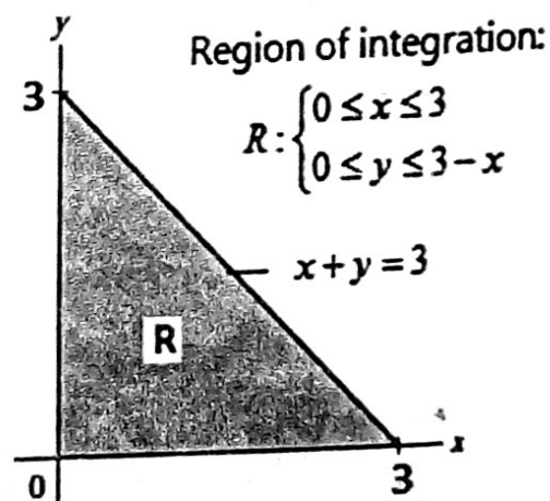
The region of integration in the xy -plane
