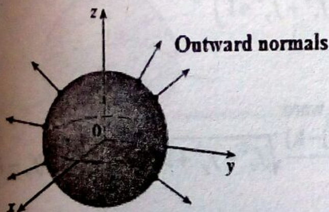
i) Positive orientation
