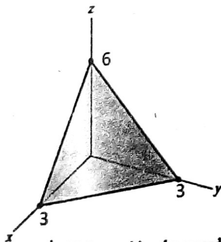
The solid formed by the coordinate axes and the plane 2x + 2y + z = 6
