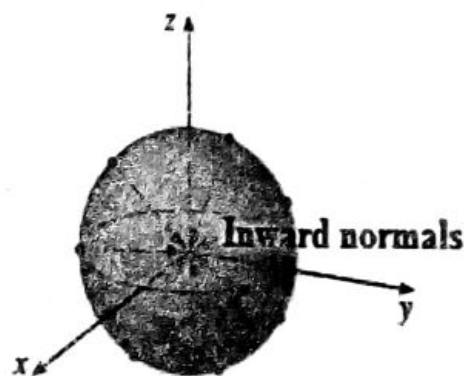
ii) Negative orientation
