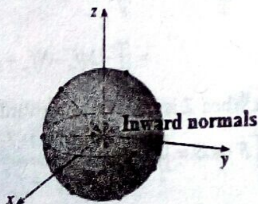
ii) Negative orientation
