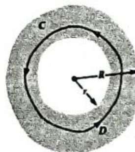
b) The contour C
