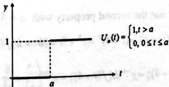
Graph of U_a(t) = U(t-a)
