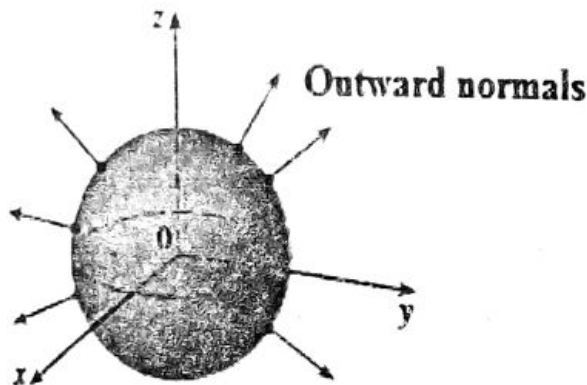
i) Positive orientation
